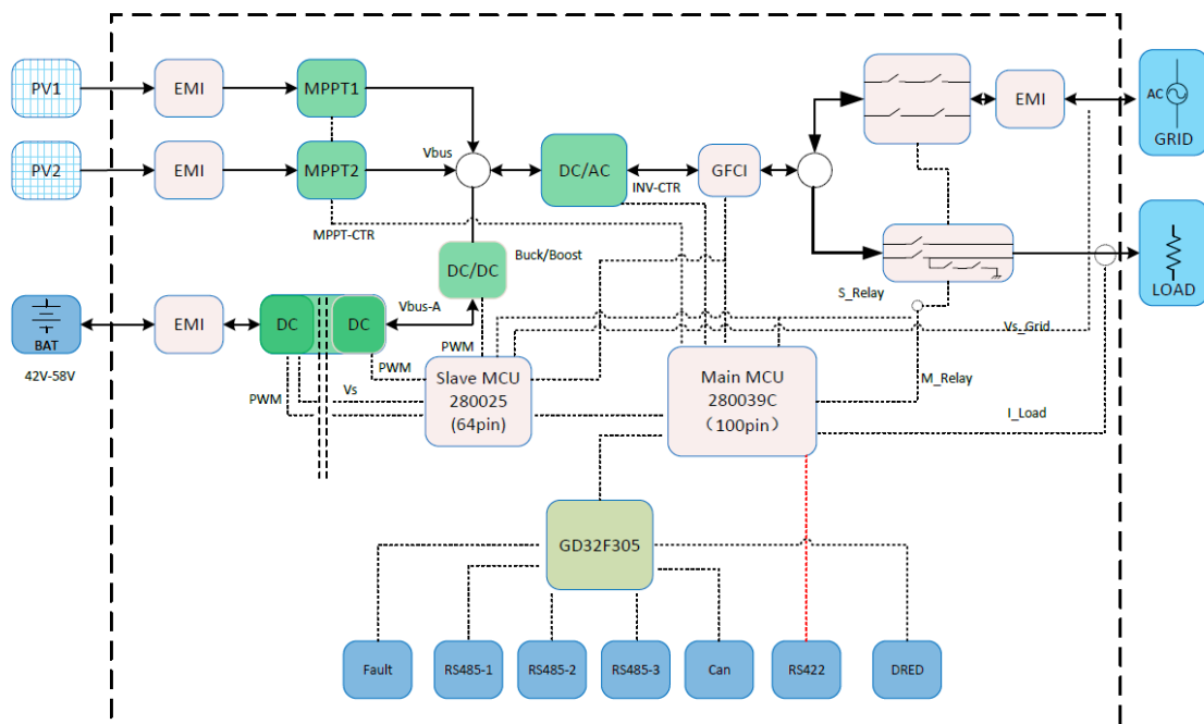
Block diagram
